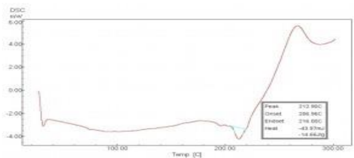
Figure 3: DSC of drug and all excipients (RSD3).
